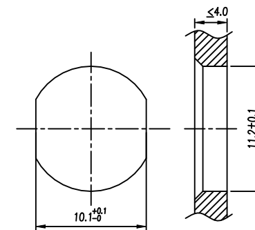
Panel cut-out
